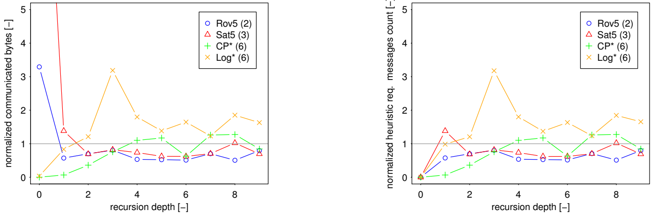
Figure 2: Communicated bytes and heuristic message requests normalized to \delta_{max} = \infty for h_{lazyFF} heuristics.
